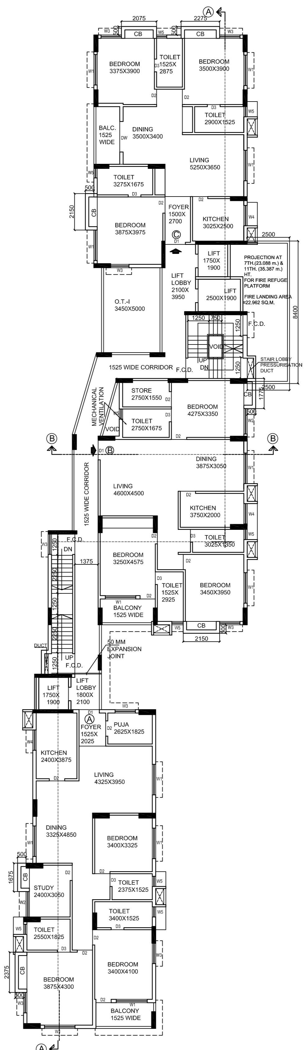
7TH. & 11TH. FLOOR PLAN. (SCALE = 1:100)
